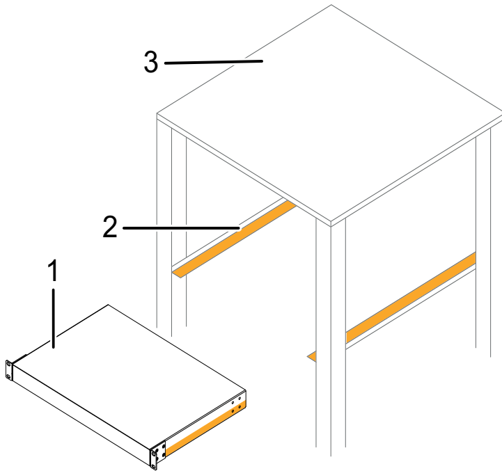
Figure 18: Assembly in a switch cabinet with sliding/mounting rails 1 - MACH1000 device 2 - sliding/mounting rail 3 - 19" switch cabinet
