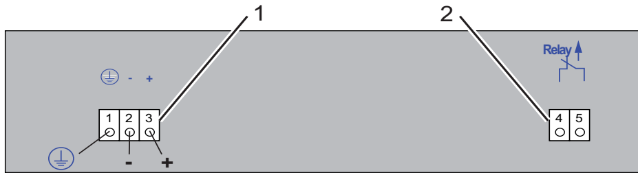
Figure 12: Power supply unit C, DC voltage ( “General technical data” on page 53 )
