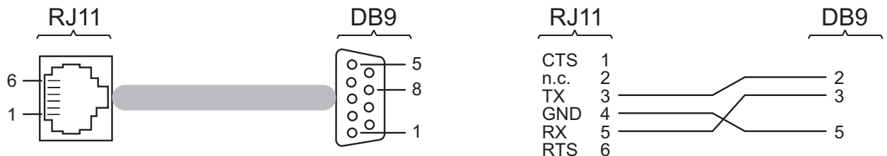
Figure 10: Pin assignment of the V.24 interface and the DB9 plug
