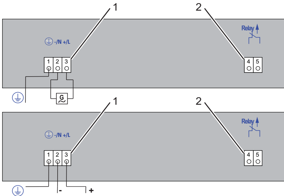
Figure 13: Power supply unit G ( see on page 53 “General technical data” ):
