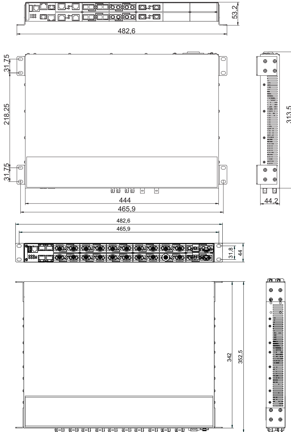
Figure 21: MACH1000, dimensions of the device variants
